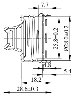
SECTION F-F
